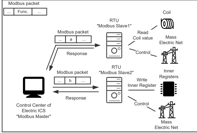
Fig. 1. Electrical ICS running Modbus protocol.
